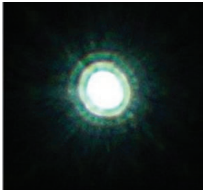
Figure 1 – Airy disk
