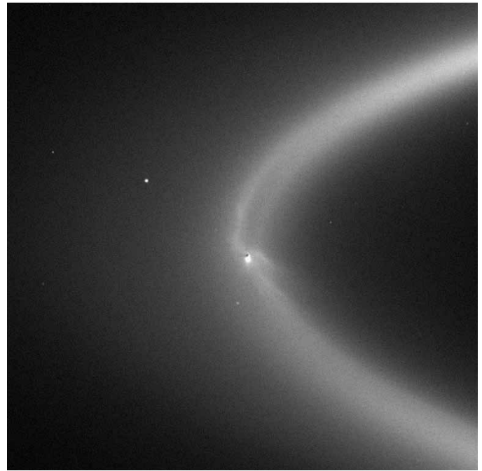
Figure 3 — Enceladus embedded in the E ring, showing wispy ice crystal plumes spewing from the moon's south pole into Saturn's E ring. (Image courtesy NASA and the creative commons on Wikipedia).
